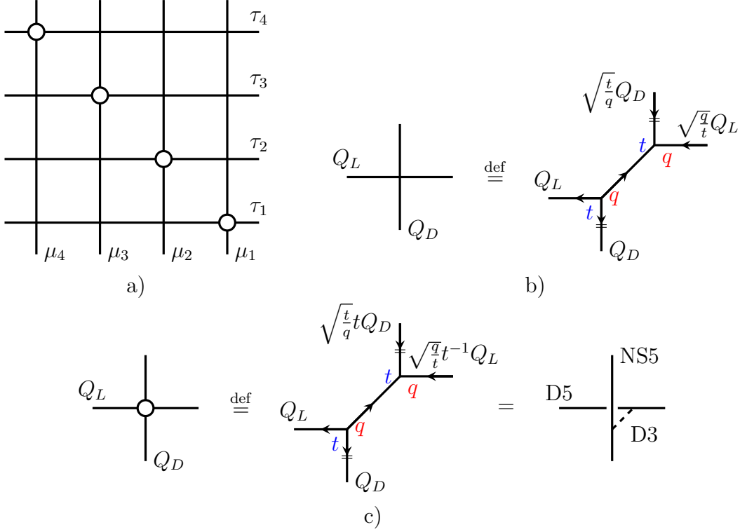
Figure 8. a) The toric diagram \mathcal{S} for the higgsed gauge theory, i.e. for parameters tuned as in Eq. (3.8). We have rotated the picture compared to Fig. 6 by \frac{\pi}{2} to aid explicit refined topological string computations. b) The “empty crossing” denotes the fully degenerate refined conifold amplitude. c) The “higgsed crossing” denote refined conifold amplitude corresponding to the geometric transition of the deformed geometry with a single brane wrapping S^3 .
