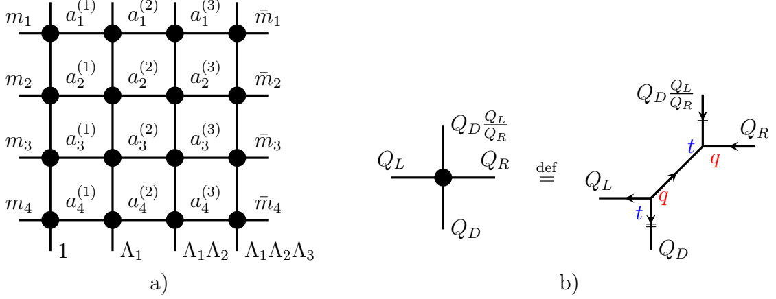
Figure 7. a) The toric diagram \mathfrak{S} producing the square gauge theory from Fig. 5. The labels of the lines correspond to the spectral parameters on the toric diagram and encode the parameters of the gauge theory. b) The shorthand notation for the crossings: black circles denote the resolved conifold geometries with general Kähler parameters. Notice that the spectral parameter on the upper vertical leg is determined by the “conservation law”.
