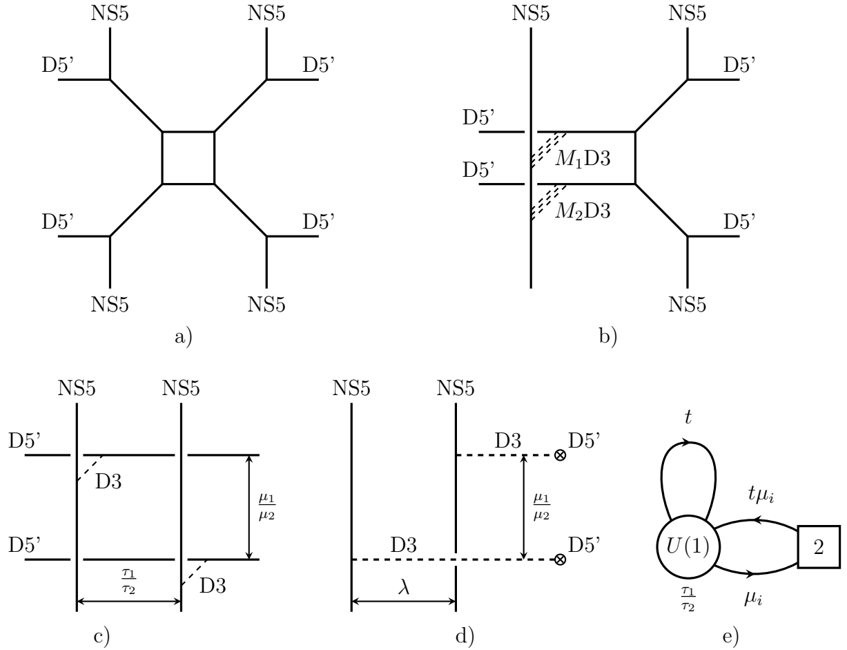
Figure 6. a) (p, q) -brane web \mathfrak{S} , corresponding to the 5d U(2) square gauge theory. The picture can also be viewed as the toric diagram of the CY. Compactifying M-theory on this CY one arrives at the same gauge theory. b) One NS5 brane is separated in the transverse direction, so that the gauge theory goes onto the Higgs branch. The dashed lines denote two stacks of M_1 and M_2 D3 branes respectively stretching between the NS5 and D5' branes. One can also view this picture as describing the CY background after the geometric transition. c) The brane setup corresponding to the 3d FT[SU(2)] theory where M_1 = 1 and M_2 = 0 . The masses \mu_{1,2} and FI parameters \tau_{1,2} of the gauge theory are encoded in the positions of the branes as shown. Notice that the second NS5 brane is also detached from the web and a single D3 is stretched between it and the second D5' brane. This imposes the condition \bar{\mu}_i = t\mu_i . d) Another projection of the brane setup c). The distance between the NS5 branes in the transversal directions \lambda corresponds to the coupling constant of the 3d theory which does not enter the holomorphic block. e) The 3d FT[SU(2)] gauge theory obtained from the brane setup c), d). The deformation parameter t giving mass to the adjoint multiplet originates from the \Omega -background in the \mathbb{R}_{q,t}^4 part of the 10d geometry.
