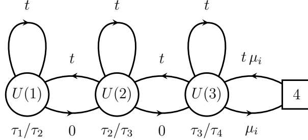
Figure 4. 3d T[SU(4)] gauge theory. \tau_a are the FI parameters. The masses of the chirals are indicated over or under the corresponding arrows.
